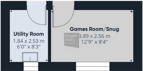
Ground floor Building 2
